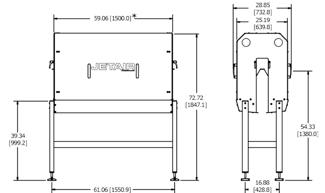
DL1500 Spray Shield
