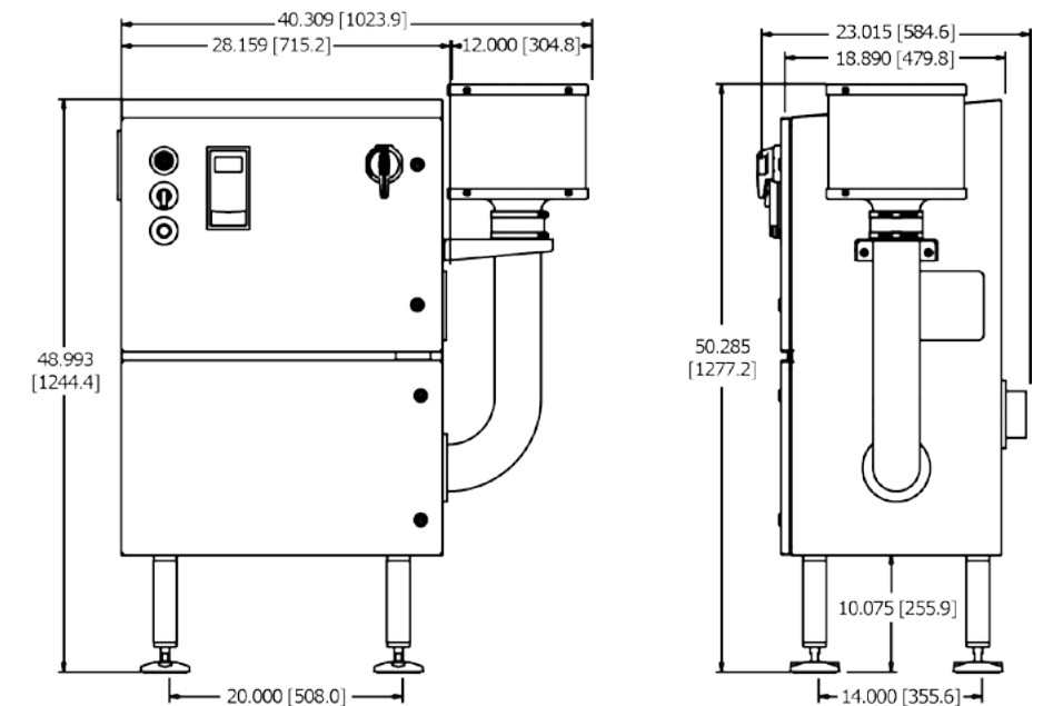
DL1500 Spray Shield
